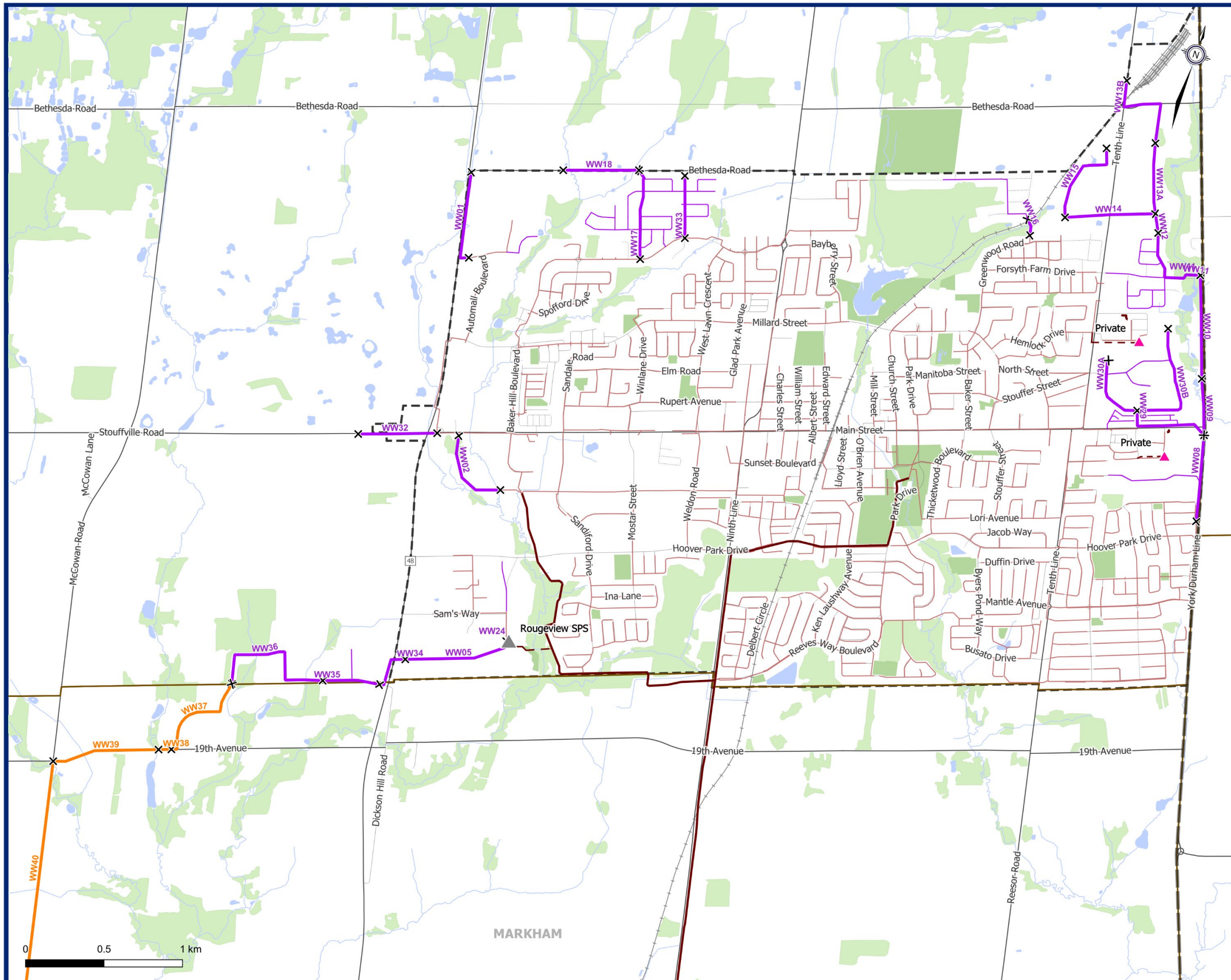
Community of Stouffville Preferred Wastewater Servicing Strategy
